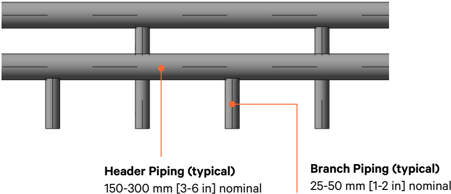
Underfloor designs for piping should leave adequate space for piping, insulation, and pipe crossover. Dimension will vary from site to site.
