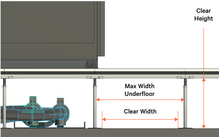
This illustration depicts the clearance required to accommodate underground piping in a facility with a raised-floor design. Dimensions will vary from site to site.
