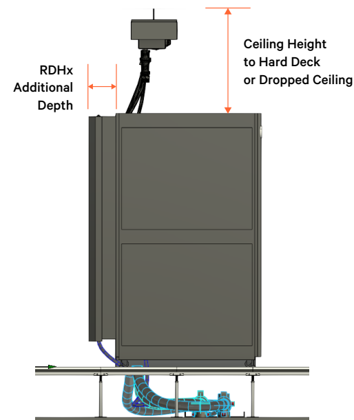
This illustration shows how running a rear-door heat exchanger adds depth to racks.
